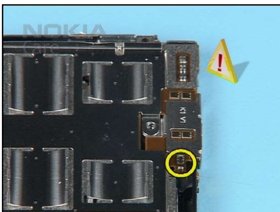
18. Take special care to the electric components on the AV FLEX.
